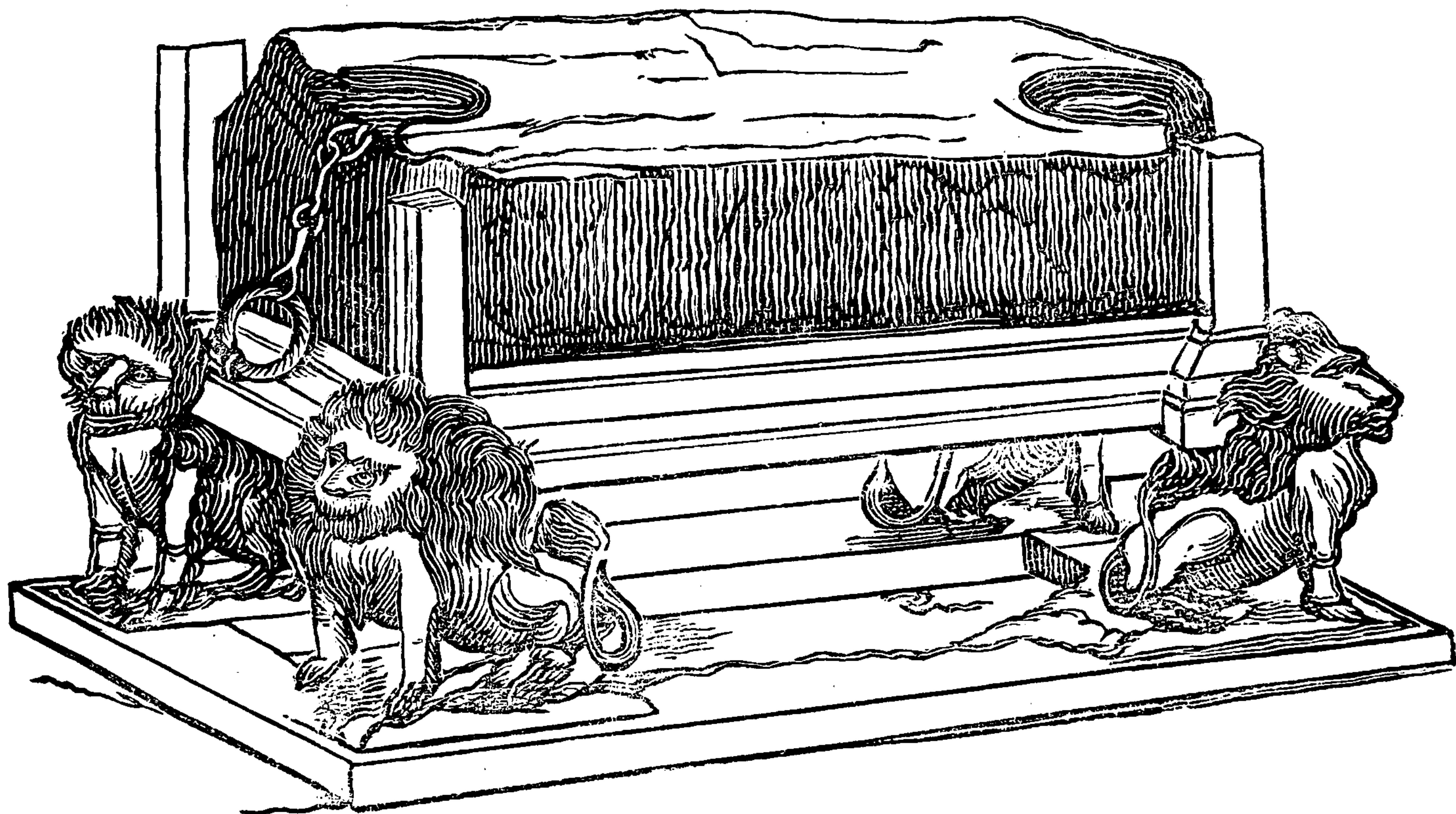
JACOB'S STONE.
